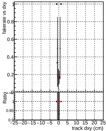
Legend for Fake rate vs dxy, Duplicates Rate vs Dxy, and Pileup rate vs dxy plots: Global (black line) mkFit batchCAND-adjusted (blue line) DCM V0001 R000000001 (red line)
