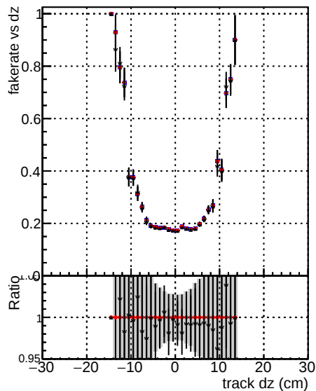
Fake rate vs d - - - /CMSSW_12_4_0_pre3/src/DQM_V0001_R000000001_Global_mkFit_batchCAND-adjusted - - - /CMSSW_12_4_0_pre3/src/DQM_V0001_R000000001_Global_mkFit_CAND - - - DQM_V0001_R000000001_Global_mkFit_CAND-AFTERCONFLICT2
