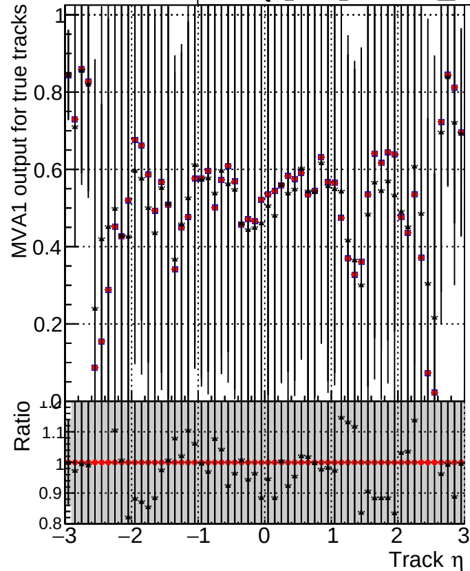
MVA1 of associated tracks (recoToSim) vs. track \eta Legend: \blacksquare ../CMSSW_12_4_0_pre3/src/DQM_V0001_R000000001_Global_mkFit_batchCAND-adjusted \bullet ../CMSSW_12_4_0_pre3/src/DQM_V0001_R000000001_Global_mkFit_CAND \blacktriangledown DQM_V0001_R000000001_Global_mkFit_CAND-AFTERCONFLICT2
