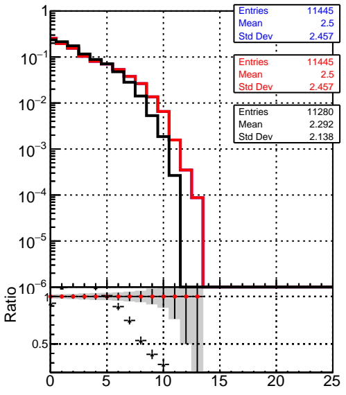
mean hit ././CMSSW_12_4_0_pre3/src/DQM_V0001_R000000001_Global_mkFit_batchCAND-adjusted ././CMSSW_12_4_0_pre3/src/DQM_V0001_R000000001_Global_mkFit_CAND DQM_V0001_R000000001_Global_mkFit_CAND-AFTERCONFLICT2
