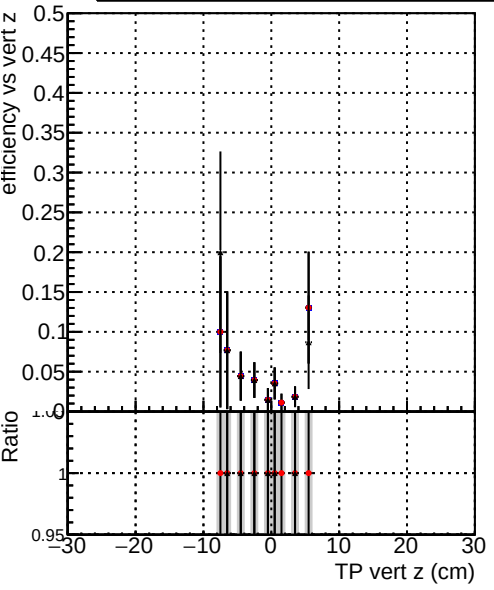
Efficiency vs vertpos Legend: ././CMSSW_12_4_0_pre3/src/DQM_V0001_R0000000001_Global_mkFit_batchCAND-adjusted ././CMSSW_12_4_0_pre3/src/DQM_V0001_R0000000001_Global_mkFit_CAND DQM_V0001_R0000000001_Global_mkFit_CAND-AFTERCONFLICT2
