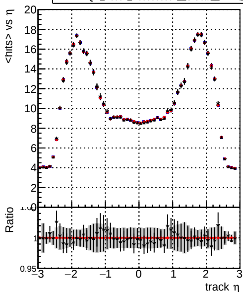
mean hits vs \eta Legend: - Blue line: ./J./CMSSW_12_4_0_pre3/src/DQM_V0001_R0000000001_Global_mkFit_batchCAND-adjusted - Red line: ./J./CMSSW_12_4_0_pre3/src/DQM_V0001_R0000000001_Global_mkFit_CAND - Black line: DQM_V0001_R0000000001_Global_mkFit_CAND-AFTERCONFLICT2
