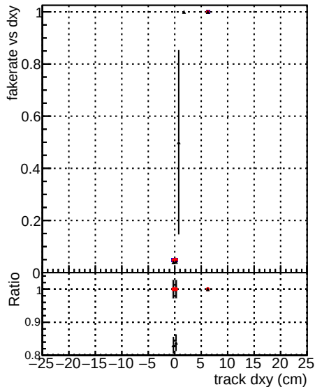
Legend for Fake rate vs dxy, Duplicates Rate vs Dxy, and Pileup rate vs dxy: Black line: /CMSSW_12_4_0_pre3/src/DQM_V0001_R0000000001_Global_mkFit_batchCAND-adjusted Red line: /CMSSW_12_4_0_pre3/src/DQM_V0001_R0000000001_Global_mkFit_CAND Black line: DQM_V0001_R0000000001_Global_mkFit_CAND-AFTERCONFLICT2
