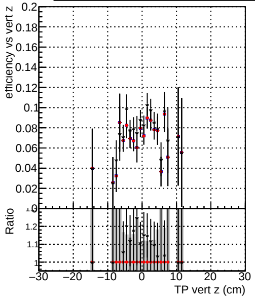
Efficiency vs vertpos Legend: Blue line: ./../CMSSW_12_4_0_pre3/src/DQM_V0001_R0000000001_Global_mkFit_batchCAND-adjusted Red line: ./../CMSSW_12_4_0_pre3/src/DQM_V0001_R0000000001_Global_mkFit_CAND Black line: DQM_V0001_R0000000001_Global_mkFit_CAND-AFTERCONFLICT
