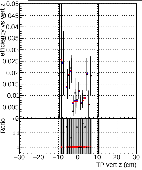
Efficiency vs vertpos Legend: Blue line with dots: ././CMSSW_12_4_0_pre3/src/DQM_V0001_R0000000001_Global_mkFit_batchCAND-adjusted Red line with dots: ././CMSSW_12_4_0_pre3/src/DQM_V0001_R0000000001_Global_mkFit_CAND Black line with dots: DQM_V0001_R0000000001_Global_mkFit_CAND-AFTERCONFLICT
