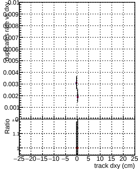
Legend for Fake rate vs d, Duplicates Rate vs Dxy, and Pileup rate vs dxy plots: Black line: /CMSSW_12_4_0_pre3/src/DQM_V0001_R000000001_Global_mkFit_batchCAND-adjusted Red line: /CMSSW_12_4_0_pre3/src/DQM_V0001_R000000001_Global_mkFit_CAND Black line: DQM_V0001_R000000001_Global_mkFit_CAND-AFTERCONFLICT
