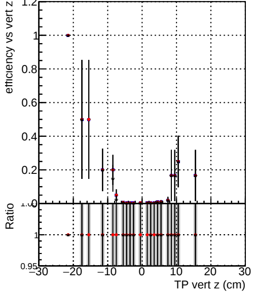
Efficiency vs vert z Legend: - ././CMSSW_12_4_0\_pre3/src/DQM_V0001_R0000000001\_Global\_mkFit\_batchCAND-adjusted - ././CMSSW_12_4_0\_pre3/src/DQM_V0001_R0000000001\_Global\_mkFit\_CAND - DQM_V0001_R0000000001\_Global\_mkFit\_CAND-AFTERCONFLICT
