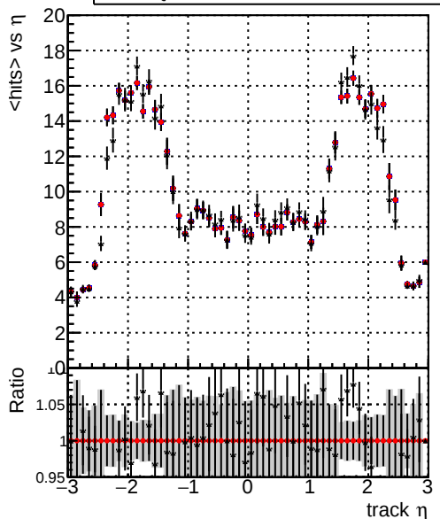
mean hit ././CMSSW_12_4_0_pre3/src/DQM_V0001_R000000001_Global_mkFit_batchCAND-adjusted ././CMSSW_12_4_0_pre3/src/DQM_V0001_R000000001_Global_mkFit_CAND DQM_V0001_R000000001_Global_mkFit_CAND-AFTERCONFLICT
