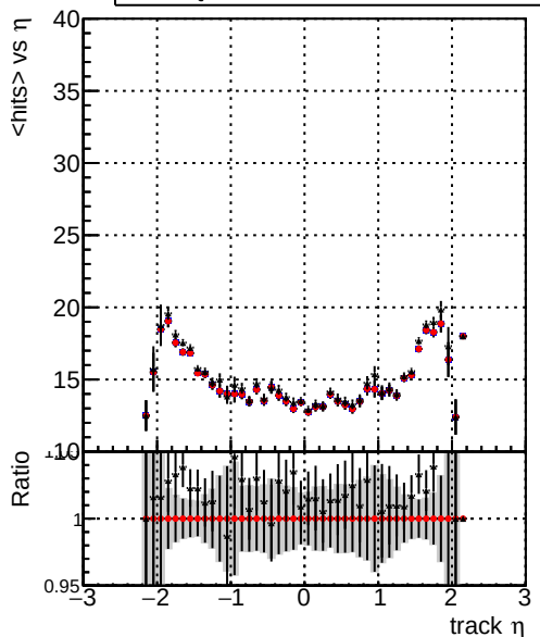
mean hits vs \eta - - - Global_mkFit_batchCAND-adjusted - - - Global_mkFit_CAND - - - DQM_V0001_R000000001_Global_mkFit_CAND-AFTERCONFLICT
