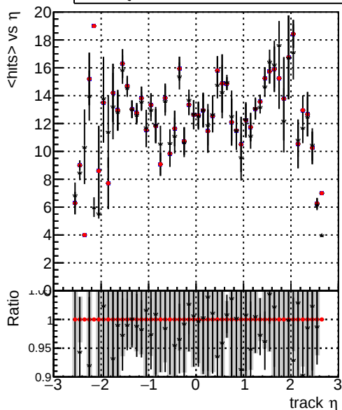
mean hit - - - Global_mkFit_batchCAND-adjusted - - - Global_mkFit_CAND - - - Global_mkFit_CAND-AFTERCONFLICT
