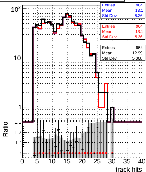
mean hit - - - Global_mkFit_batchCAND-adjusted - - - Global_mkFit_CAND - - - Global_mkFit_CAND-AFTERCONFLICT
