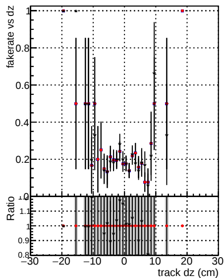
Fake rate vs dz - - - /CMSSW_12_4_0_pre3/src/DQM_V0001_R000000001_Global_mkFit_batchCAND-adjusted - - - /CMSSW_12_4_0_pre3/src/DQM_V0001_R000000001_Global_mkFit_CAND - - - DQM_V0001_R000000001_Global_mkFit_CAND-AFTERCONFLICT
