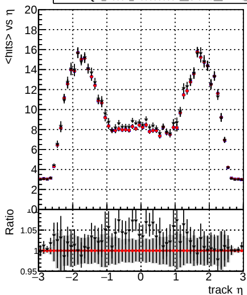
mean hits vs \eta Legend: - Blue line: ././CMSSW_12_4_0_pre3/src/DQM_V0001_R0000000001_Global_mkFit_batchCAND-adjusted - Red line: ././CMSSW_12_4_0_pre3/src/DQM_V0001_R0000000001_Global_mkFit_CAND - Black line: DQM_V0001_R0000000001_Global_mkFit_CAND-AFTERCONFLICT
