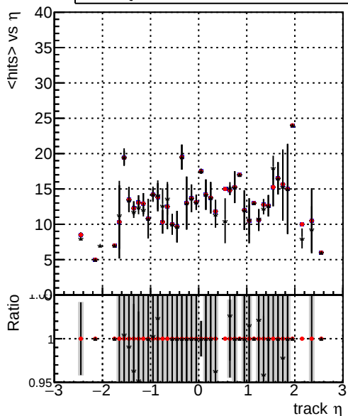
mean hits vs \eta Legend: - Blue line: ./../CMSSW_12_4_0_pre3/src/DQM_V0001_R000000001_Global_mkFit_batchCAND-adjusted - Red line: ./../CMSSW_12_4_0_pre3/src/DQM_V0001_R000000001_Global_mkFit_CAND - Black line: DQM_V0001_R000000001_Global_mkFit_CAND-AFTERCONFLICT
