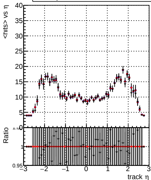
mean hit ..../CMSSW_12_4_0_pre3/src/DQM_V0001_R000000001_Global_mkFit_batchCAND-adjusted ..../CMSSW_12_4_0_pre3/src/DQM_V0001_R000000001_Global_mkFit_CAND DQM_V0001_R000000001_Global_mkFit_CAND-AFTERCONFLICT
