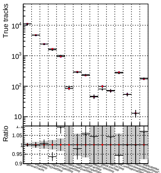
Number Legend Blue line with square: ../CMSSW_12_4_0_pre3/src/DQM_V0001_R0000000001_Global_mkFit_batchCAND-adjusted Red line with circle: ../CMSSW_12_4_0_pre3/src/DQM_V0001_R0000000001_Global_mkFit_CAND Black line with triangle: DQM_V0001_R0000000001_Global_mkFit_CAND-AFTERCONFLICT
