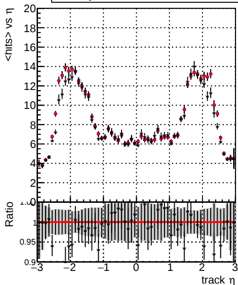
mean hit ..../CMSSW_12_4_0_pre3/src/DQM_V0001_R0000000001_Global_mkFit_batchCAND-adjusted ..../CMSSW_12_4_0_pre3/src/DQM_V0001_R0000000001_Global_mkFit_CAND DQM_V0001_R0000000001_Global_mkFit_CAND-AFTERCONFLICT
