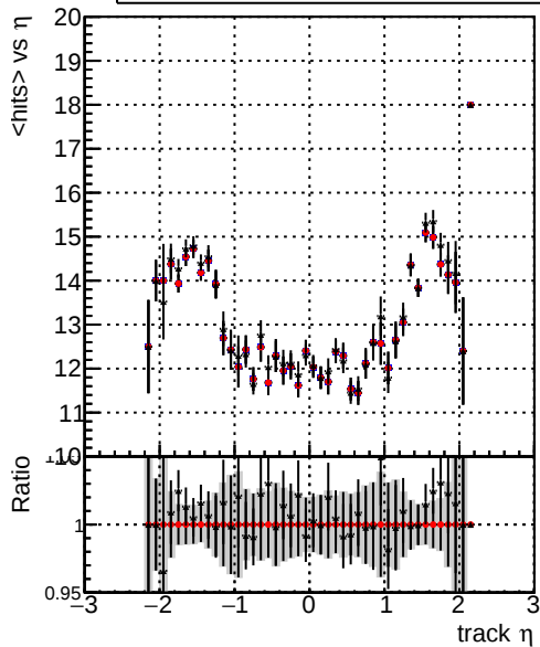
mean hit ./../CMSSW_12_4_0_pre3/src/DQM_V0001_R000000001_Global_mkFit_batchCAND-adjusted ./../CMSSW_12_4_0_pre3/src/DQM_V0001_R000000001_Global_mkFit_CAND DQM_V0001_R000000001_Global_mkFit_CAND-AFTERCONFLICT
