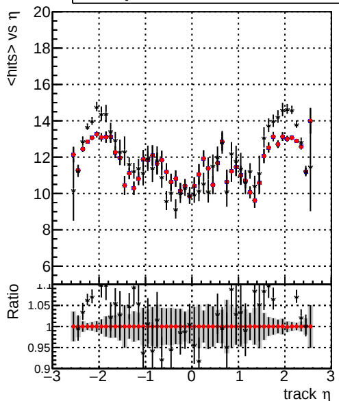
mean hit \frac{DQM\_V0001\_R000000001\_Global\_mkFit\_batchCAND-adjusted}{DQM\_V0001\_R000000001\_Global\_mkFit\_CAND} \frac{DQM\_V0001\_R000000001\_Global\_mkFit\_CAND-AFTERCONFLICT}{DQM\_V0001\_R000000001\_Global\_mkFit\_CAND}
