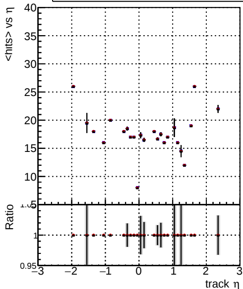
mean hits > \eta Legend: - Blue line: ./J/CMSSW_12_4_0_pre3/src/DQM_V0001_R000000001_Global_mkFit_batchCAND-adjusted - Red line: ./J/CMSSW_12_4_0_pre3/src/DQM_V0001_R000000001_Global_mkFit_CAND - Black line: DQM_V0001_R000000001_Global_mkFit_CAND-AFTERCONFLICT
