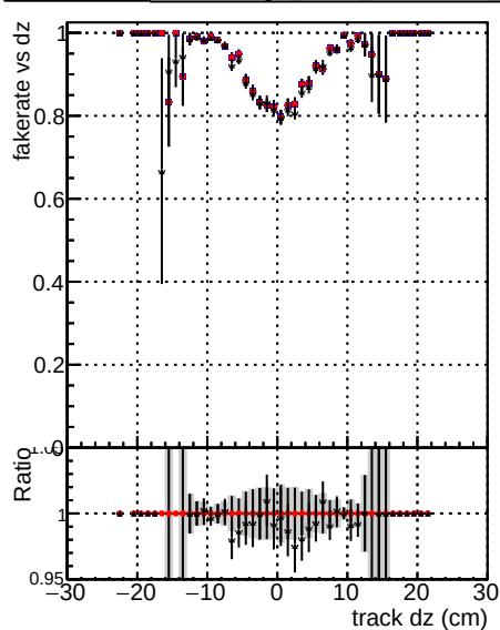
Fake rate vs d ../CMSSW_12_4_0_pre3/src/DOM_V0001_R0000000001_Global_mkFit_batchCAND-adjusted ../CMSSW_12_4_0_pre3/src/DOM_V0001_R0000000001_Global_mkFit_CAND DOM_V0001_R0000000001_Global_mkFit_CAND-AFTERCONFLICT
