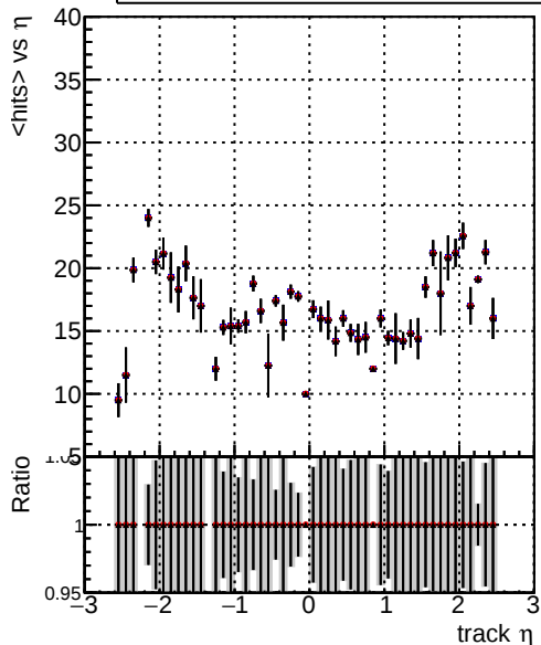
mean hits ..../CMSSW_12_4_0_pre3/src/DQM_V0001_R0000000001_Global_mkFit_batchCAND-adjusted ..../CMSSW_12_4_0_pre3/src/DQM_V0001_R0000000001_Global_mkFit_CAND DQM_V0001_R0000000001_Global_mkFit_CAND-AFTERCONFLICT
