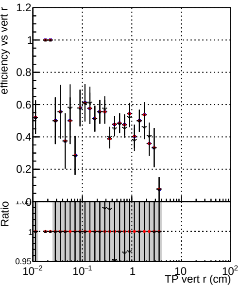
Efficiency vs TP vert r (cm) Legend: ././CMSSW_12_4_0_pre3/src/DQM_V0001_R0000000001_Global_mkFit_batchCAND-adjusted ././CMSSW_12_4_0_pre3/src/DQM_V0001_R0000000001_Global_mkFit_CAND DQM_V0001_R0000000001_Global_mkFit_CAND-AFTERCONFLICT
