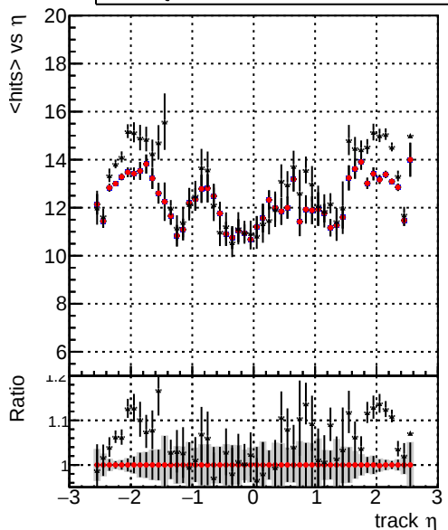
mean hits Legend: - Blue line: ././CMSSW_12_4_0_pre3/src/DQM_V0001_R0000000001_Global_mkFit_batchCAND-adjusted - Red line: ././CMSSW_12_4_0_pre3/src/DQM_V0001_R0000000001_Global_mkFit_CAND - Black line: DQM_V0001_R0000000001_Global_mkFit_CAND-AFTERCONFLICT
