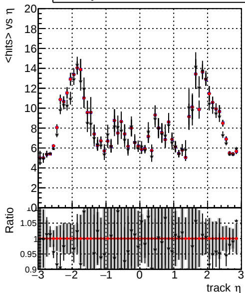
mean hit \frac{1}{N} \sum_{i=1}^N \langle \text{hits} \rangle_i vs \eta - \frac{1}{N} \sum_{i=1}^N \langle \text{hits} \rangle_i vs \eta (Global_mkFit_batchCAND-adjusted) - \frac{1}{N} \sum_{i=1}^N \langle \text{hits} \rangle_i vs \eta (Global_mkFit_CAND) - \frac{1}{N} \sum_{i=1}^N \langle \text{hits} \rangle_i vs \eta (Global_mkFit_CAND-AFTERCONFLICT)
