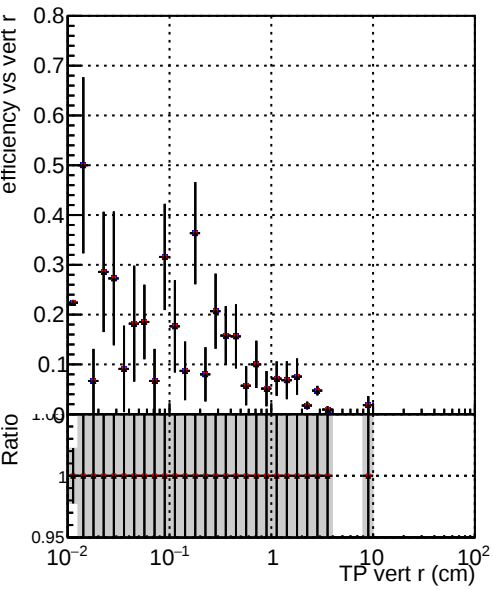
Efficiency vs vertpos —●— DQM_V0001_R000000001_Global_mkFit_noCAND —●— DQM_V0001_R000000001_Global_mkFit_CAND —●— DQM_V0001_R000000001_Global_mkFit_batchCAND-adjusted
