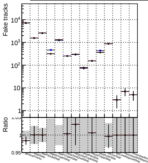
Number —●— DQM_V0001_R0000000001_Global_mkFit_CAND —★— DQM_V0001_R0000000001_Global_mkFit_batchCAND-adjusted
