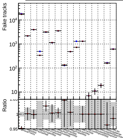
Number —●— DQM_V0001_R0000000001_Global_mkFit_CAND —★— DQM_V0001_R0000000001_Global_mkFit_batchCAND-adjusted
