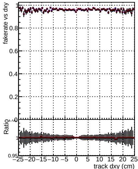
Legend for Fake rate vs d, Duplicates Rate vs Dxy, and Pileup rate vs dxy: DOM V0001 R0000000001 Global mkFit noCAND DOM V0001 R0000000001 Global mkFit CAND DOM V0001 R0000000001 Global mkFit batchCAND-adjusted
