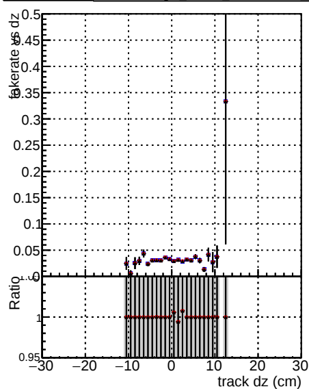
Fake rate vs dz Legend: DOM V0001 R0000000001 Global mkFit noCAND DOM V0001 R0000000001 Global mkFit CAND DOM V0001 R0000000001 Global mkFit batchCAND-adjusted
