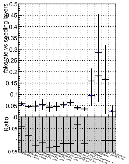
◆ DGM V0001 R0000000001 Global mkFit noCAND ● DGM V0001 R0000000001 Global mkFit CAND — DGM V0001 R0000000001 Global mkFit batchCAND-adjusted
