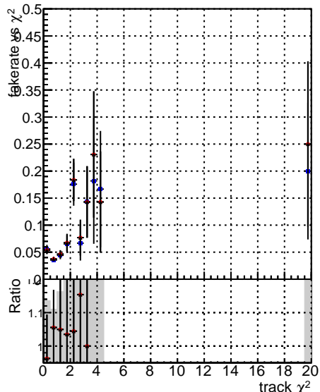
◆ DGM V0001 R0000000001 Global mkFit noCAND ● DGM V0001 R0000000001 Global mkFit CAND — DGM V0001 R0000000001 Global mkFit batchCAND-adjusted
