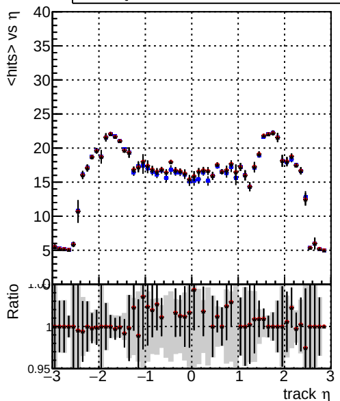
mean hits vs \eta DQM_V0001_R000000001_Global_mkFit_noCAND DQM_V0001_R000000001_Global_mkFit_CAND DQM_V0001_R000000001_Global_mkFit_batchCAND-adjusted
