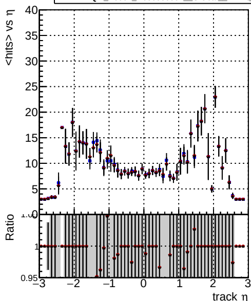
mean hits DQM_V0001_R000000001_Global_mkFit_noCAND DQM_V0001_R000000001_Global_mkFit_CAND DQM_V0001_R000000001_Global_mkFit_batchCAND-adjusted
