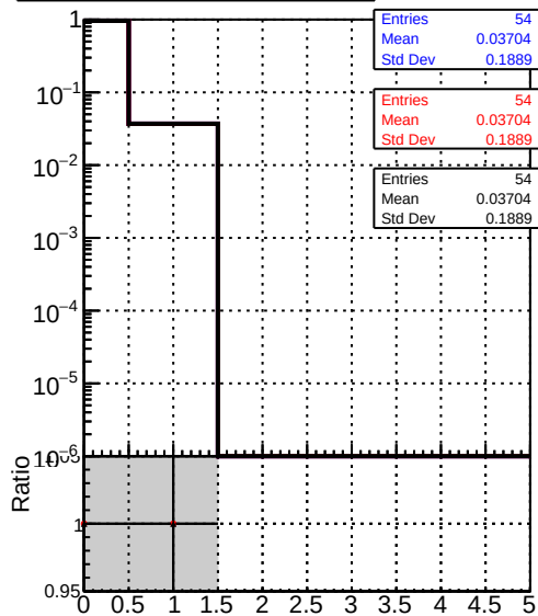
mean hit — DQM_V0001_R000000001_Global_mkFit_noCAND — DQM_V0001_R000000001_Global_mkFit_CAND — DQM_V0001_R000000001_Global_mkFit_batchCAND-adjusted
