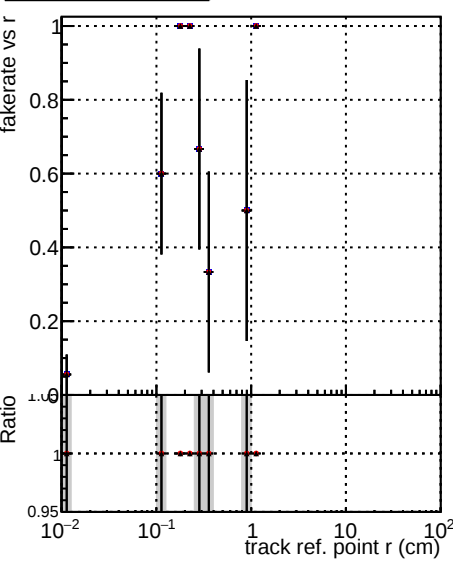
Legend: DQM_V0001_R000000001 Global mkFit_noCAND, DQM_V0001_R000000001 Global mkFit_CAND, DQM_V0001_R000000001 Global mkFit_batchCAND-adjusted
