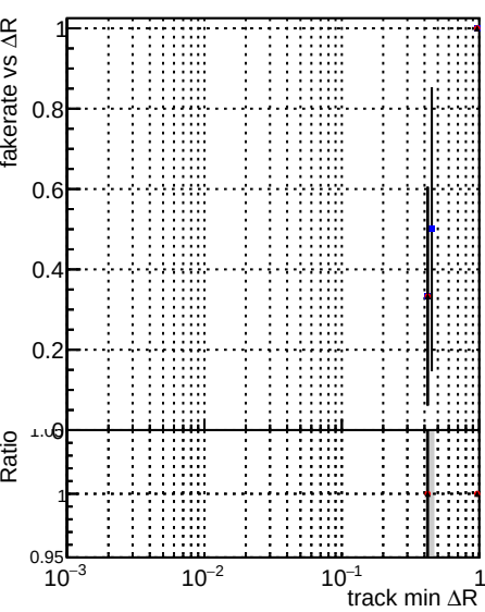
Fake rate vs ΔR(track, jet) DQM_V0001_R000000001 Global mkFit_noCAND DQM_V0001_R000000001 Global mkFit_CAND DQM_V0001_R000000001 Global mkFit_batchCAND-adjusted
