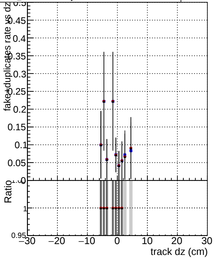
DQM_V0001_R000000001 Global mkFit_noCAND DQM_V0001_R000000001 Global mkFit_CAND DQM_V0001_R000000001 Global mkFit_batchCAND-adjusted
