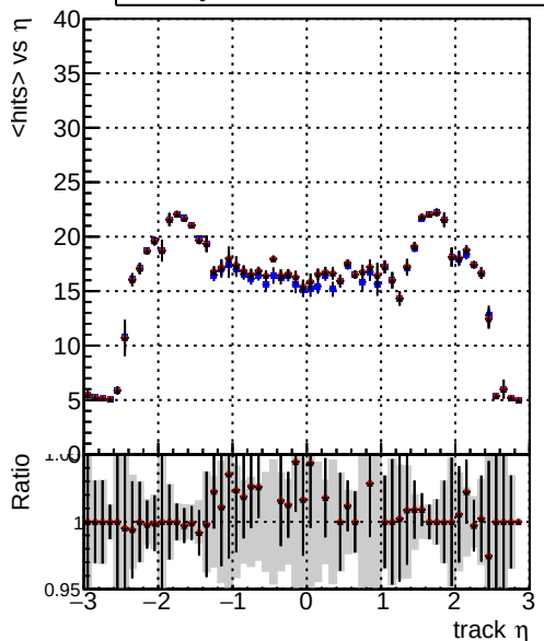
mean hits vs \eta Legend: — DQM_V0001_R000000001_Global_mkFit_noCAND (blue) — DQM_V0001_R000000001_Global_mkFit_CAND (red) — DQM_V0001_R000000001_Global_mkFit_batchCAND-adjusted (black)
