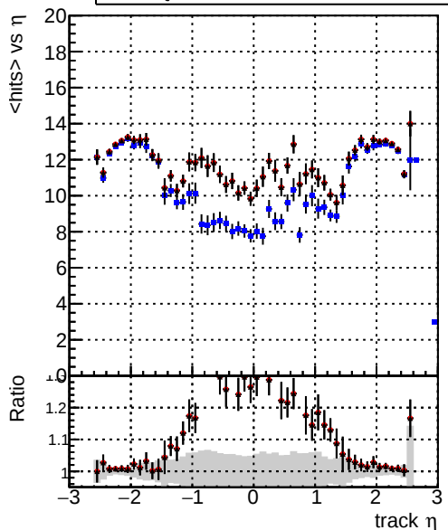
mean hit — DQM_V0001_R000000001_Global_mkFit_noCAND — DQM_V0001_R000000001_Global_mkFit_CAND — DQM_V0001_R000000001_Global_mkFit_batchCAND-adjusted
