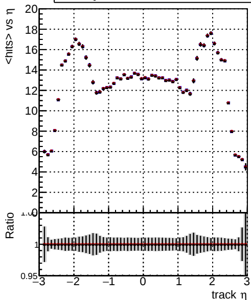
mean hits vs \eta DQM_V0001_R000000001_Global_mkFit_noCAND DQM_V0001_R000000001_Global_mkFit_CAND DQM_V0001_R000000001_Global_mkFit_batchCAND-adjusted
