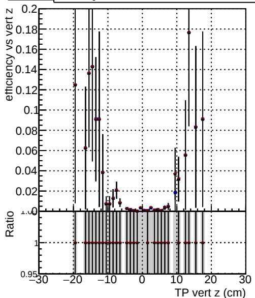
Efficiency vs. TP vert z (cm) —●— DQM_V0001_R0000000001_Global_mkFit_noCAND —●— DQM_V0001_R0000000001_Global_mkFit_CAND —●— DQM_V0001_R0000000001_Global_mkFit_batchCAND-adjusted
