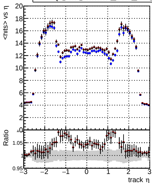
mean hits vs \eta Legend: DQM_V0001_R000000001_Global_mkFit_noCAND (blue line), DQM_V0001_R000000001_Global_mkFit_CAND (red line), DQM_V0001_R000000001_Global_mkFit_batchCAND-adjusted (black line)
