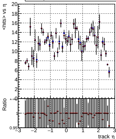
mean hits vs \eta DQM_V0001_R000000001_Global_mkFit_noCAND DQM_V0001_R000000001_Global_mkFit_CAND DQM_V0001_R000000001_Global_mkFit_batchCAND-adjusted
