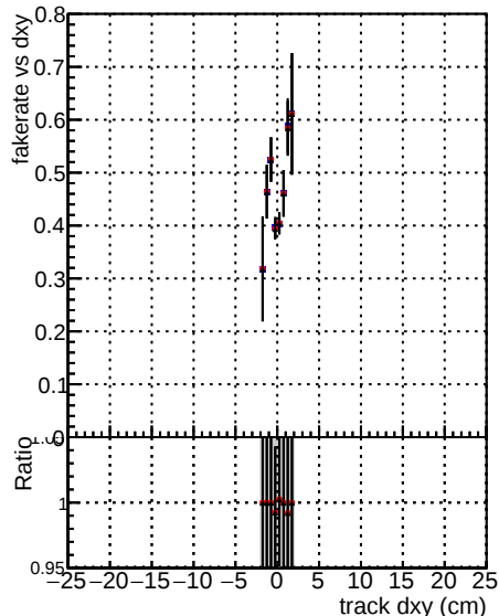
Legend for Fake rate vs dxy, Duplicates Rate vs Dxy, and Pileup rate vs dxy: Global mkFit noCAND Global mkFit CAND Global mkFit batchCAND-adjusted
