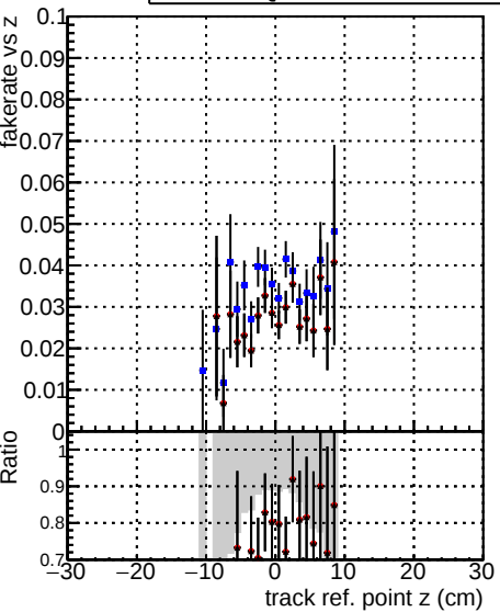
Fake rate vs verpos Legend: DQM_V0001_R000000001 Global mkFit_noCAND DQM_V0001_R000000001 Global mkFit_CAND DQM_V0001_R000000001 Global mkFit_batchCAND-adjusted
