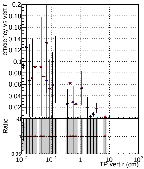
Efficiency vs vertpos Legend: DQM_V0001_R0000000001_Global_mkFit_noCAND DQM_V0001_R0000000001_Global_mkFit_CAND DQM_V0001_R0000000001_Global_mkFit_batchCAND
