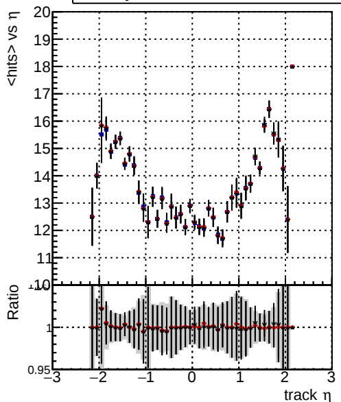
mean hits vs \eta DQM_V0001_R000000001_Global_mkFit_noCAND DQM_V0001_R000000001_Global_mkFit_CAND DQM_V0001_R000000001_Global_mkFit_batchCAND
